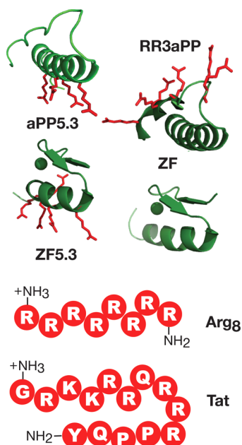
Figure 1. Examples of the peptides and protein domains evaluated in this work. Arginine side chains are shown explicitly in those molecules drawn as ribbons. 32,33
